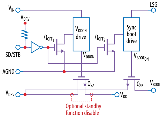
Figure 11: Simplified Circuit Diagram of V_{IN} , V_{DRV} , V_{DDX} , and V_{BOOTX} Power Supplies. Only one phase is shown.
