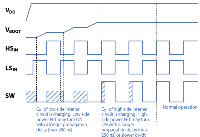
Figure 13: Behavior before complete charging of internal gate driver capacitors
